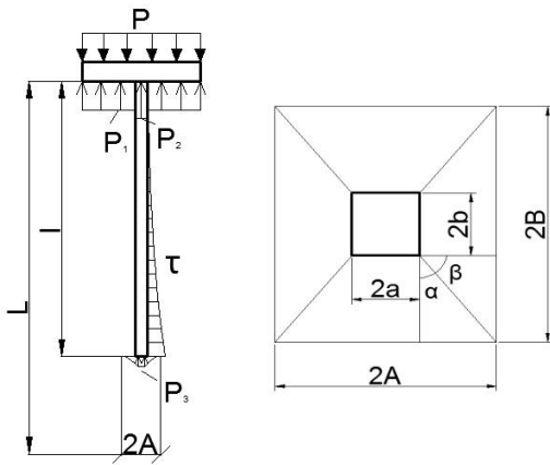
Figure 2. The calculating scheme of the interaction of a single pile with a homogeneous array of soil with a size 2A \times 2B
