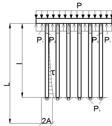
Figure 1. The calculating scheme of the interaction of plate-pile foundation with an array of soil
