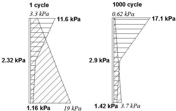
Figure 3. Distribution diagrams of mobilized tangential stress and ultimate shear stress
